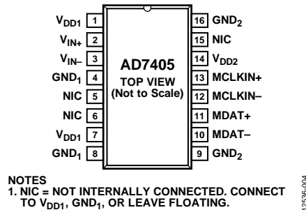
Figure 4. Pin Configuration
