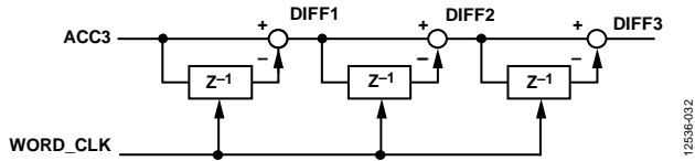
Figure 32. Differentiator
